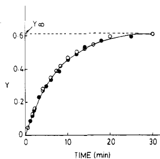
Figure 4. Course of photoisomerization of I (●) and III (○) in dilute solution. Y_\infty is the fraction of cis -azobenzene residues at the photostationary state.
