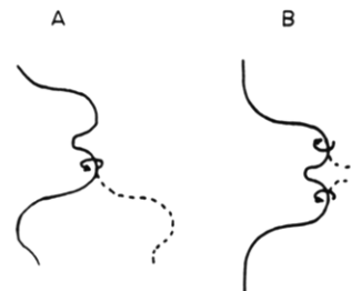
Figure 2. Schematic representation of conformational transition in a flexible chain molecule: (A) rotation around a single bond; (B) correlated rotation around two bonds.
