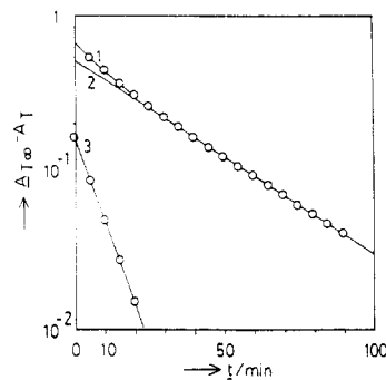
Figure 6. Resolution of the thermal cis - trans isomerization of the azo chromophore in a copolymer of ethyl methacrylate at 70 °C using two first-order reactions. A_\infty and A_t are the absorbances at \lambda = 353 nm at infinite time and at time t : (1) experimental curve; (2) normal isomerization curve; (3) fast reaction curve (Eisenbach, C. D. Makromol. Chem. 1978, 179, 2507).
